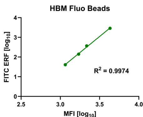
Figure 2: HansaBioMed's fluorescent bead standards measured on F-NTA.
