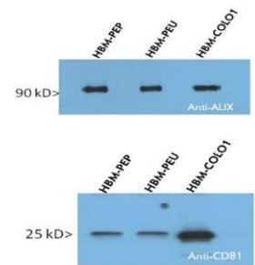
1. Western Blot comparison of exosomal markers on fresh (F), frozen (-20°C) and lyophilized exosomes (L). Particle size distribution of Exosomes stored lyophilized or frozen.
